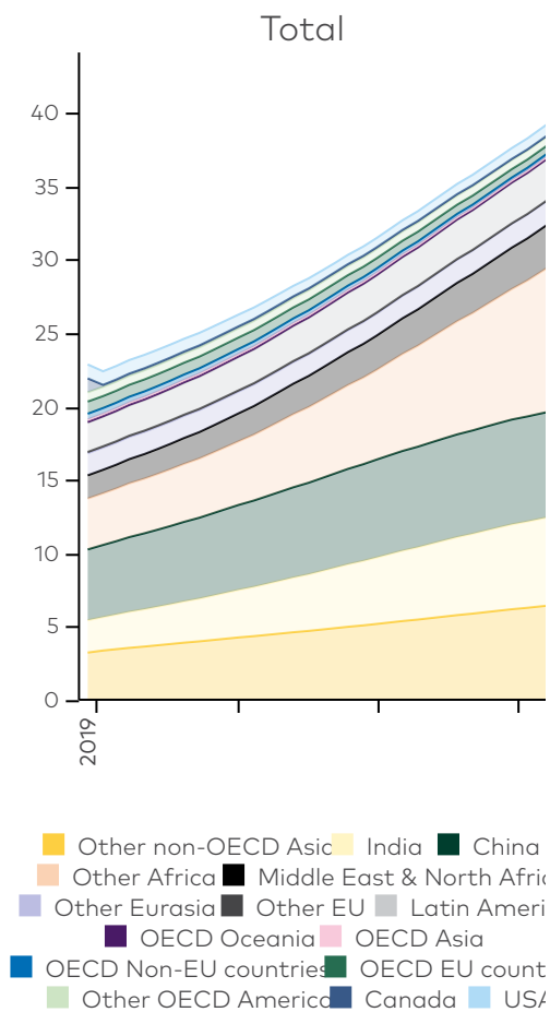
Figure A3: Estimates of plastic leakage (in million tonnes per year) from different world regions for 2019 and projected until 2060 using a business as usual scenario (OECD, 2022b).
