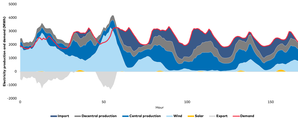
Figure 44: Electricity production distribution in the first week of 2018 in DK1, which is representative of the principle being illustrated.
