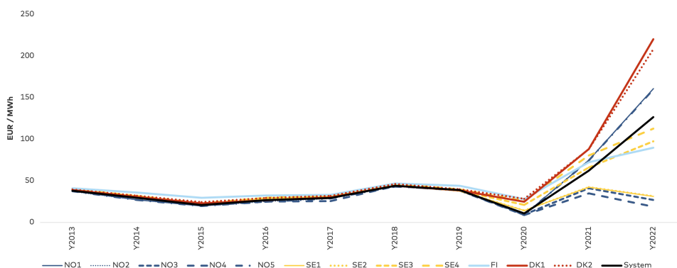
Figure 36: Annual electricity price average in the Nordic price zones.
